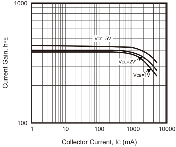
Fig.1 - Current Gain vs. Collector Current
